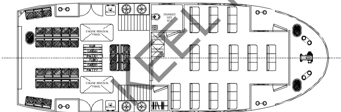
MAIN DECK
